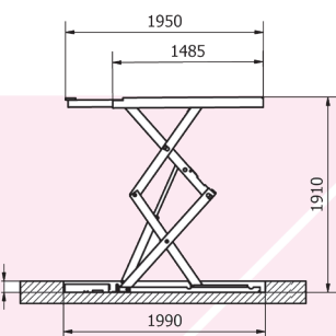
Inground version
