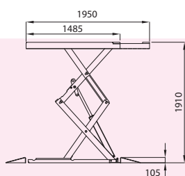
Onground version
